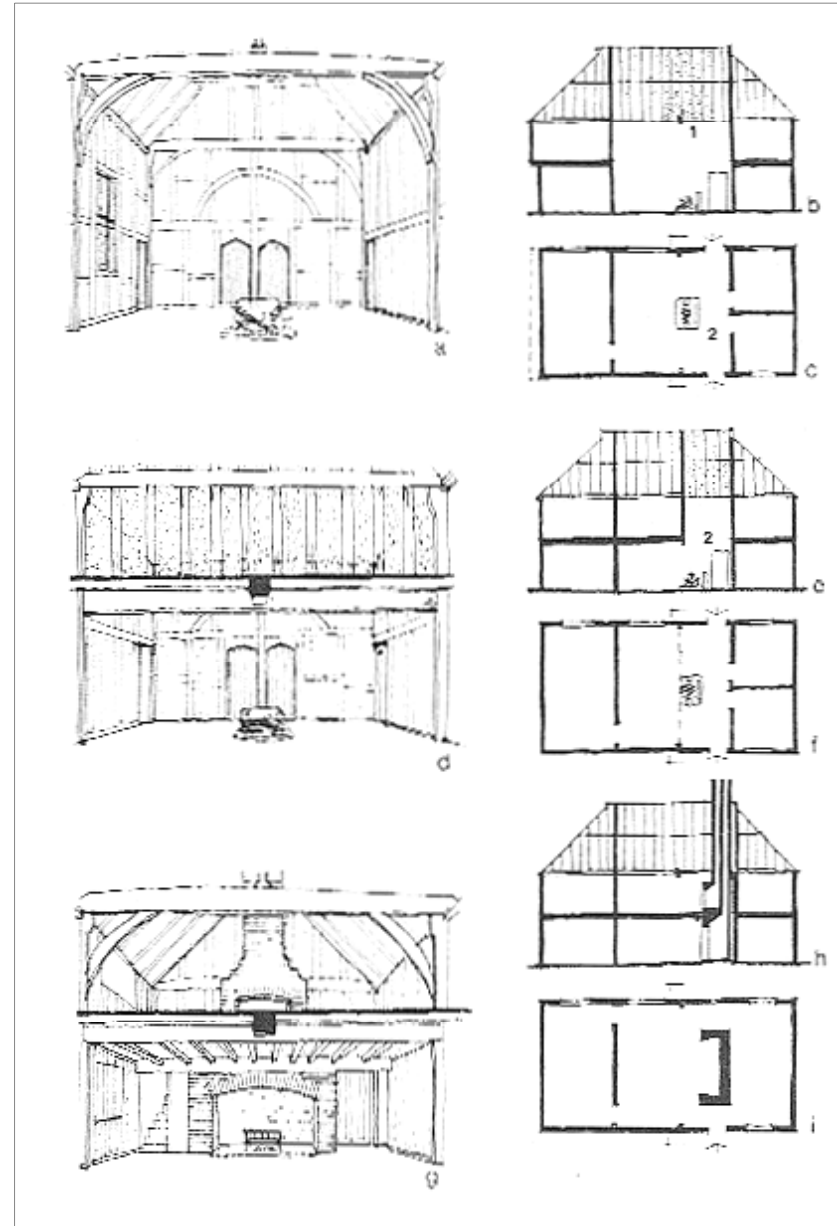
'Wealden' Hall House (left), evolving to three-unit house (right) – R. W. Brunskill, 'Houses and Cottages of Britain'
